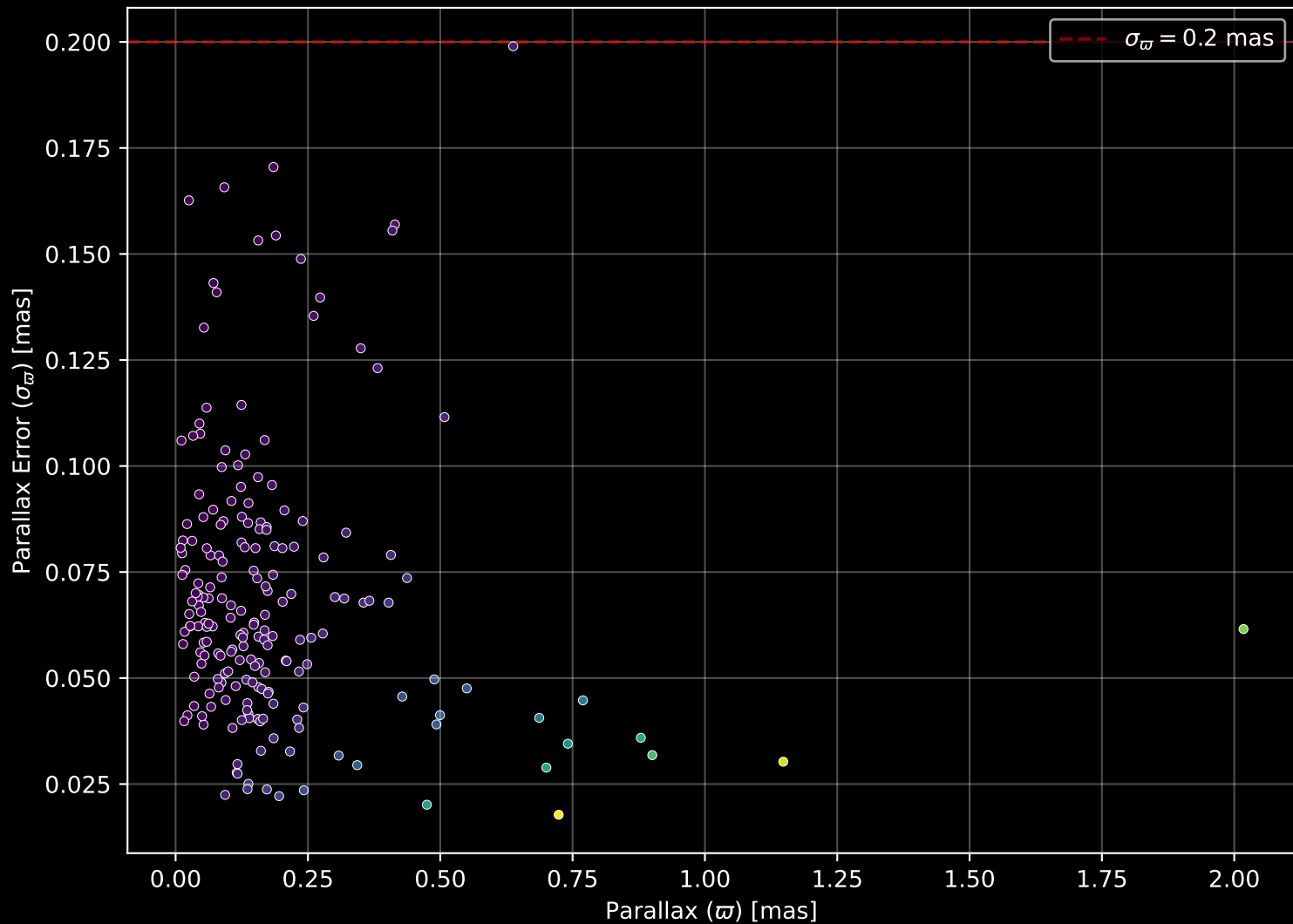
APOGEE DR17 Field: [355+04] Parallax Quality (n= 201)
