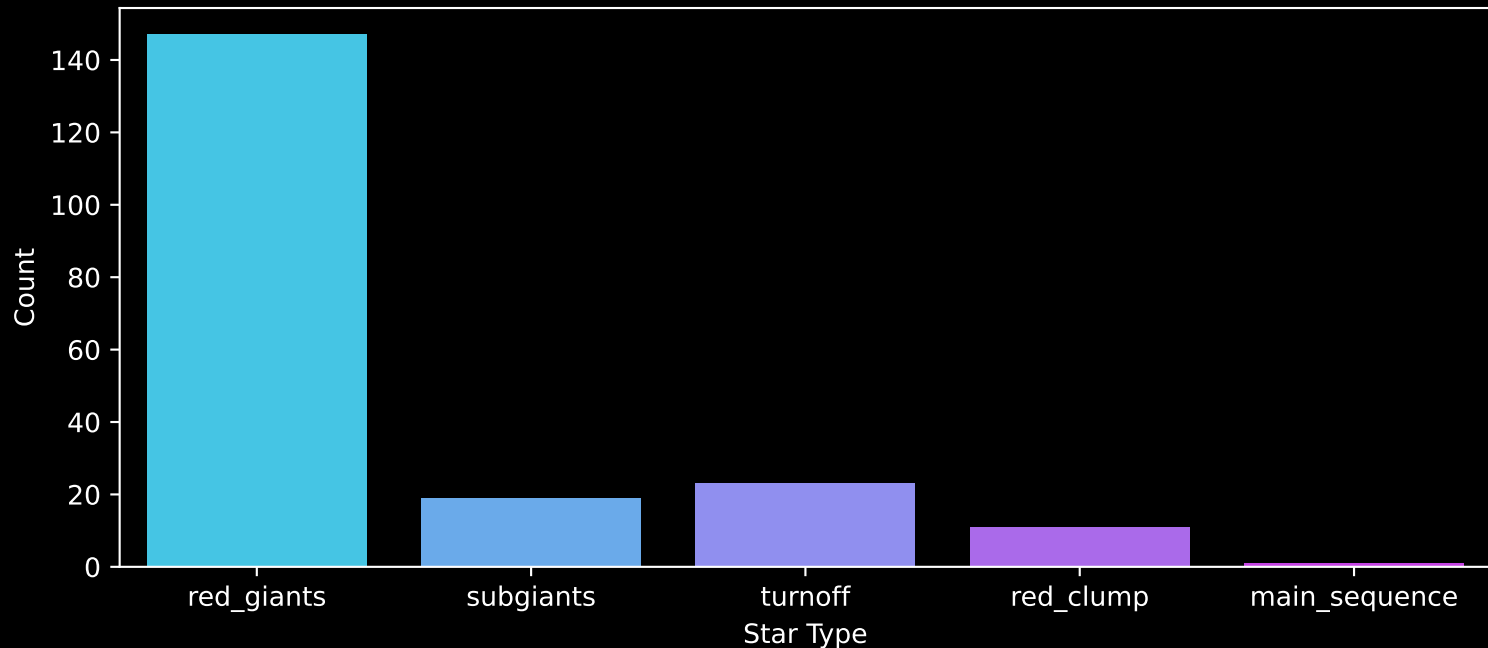
APOGEE DR17 Field: [355+04] Count plot of Star Type
