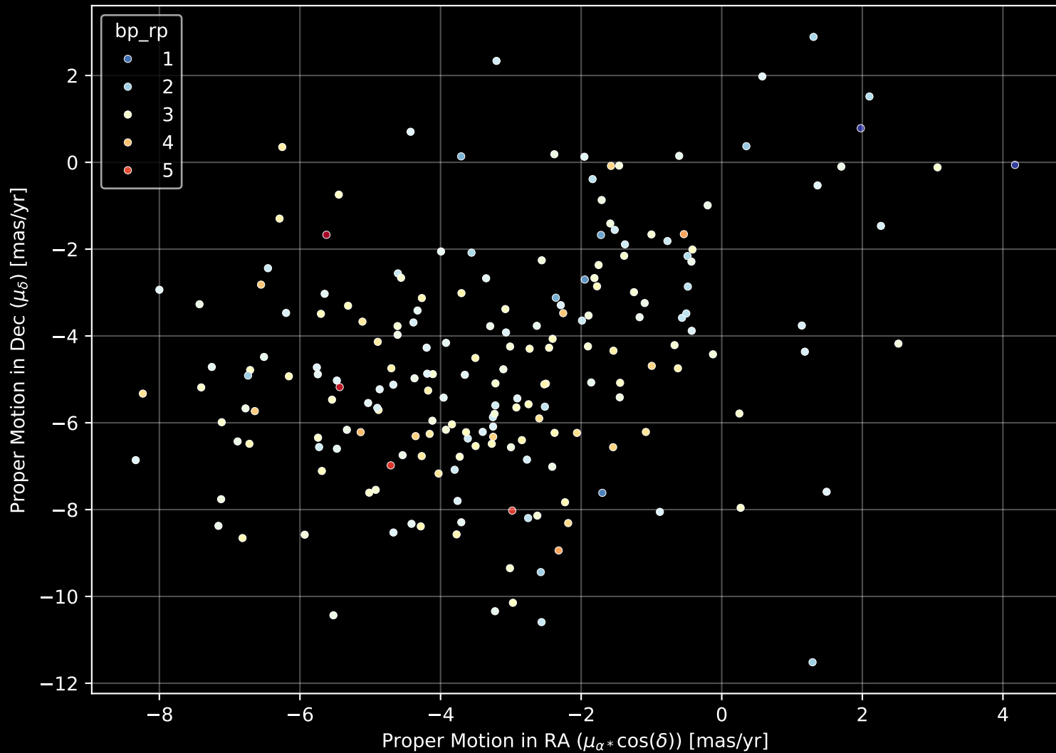
APOGEE DR17 Field: [355+04] Proper Motion Diagram (n= 201)
