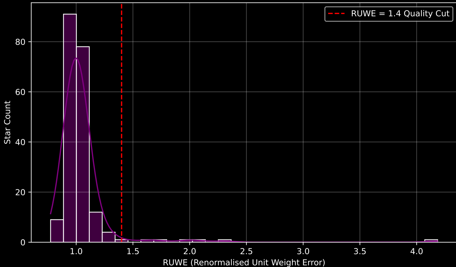
GAPOGEE DR17 Field [355+04] RUWE Distribution (n= 201)
