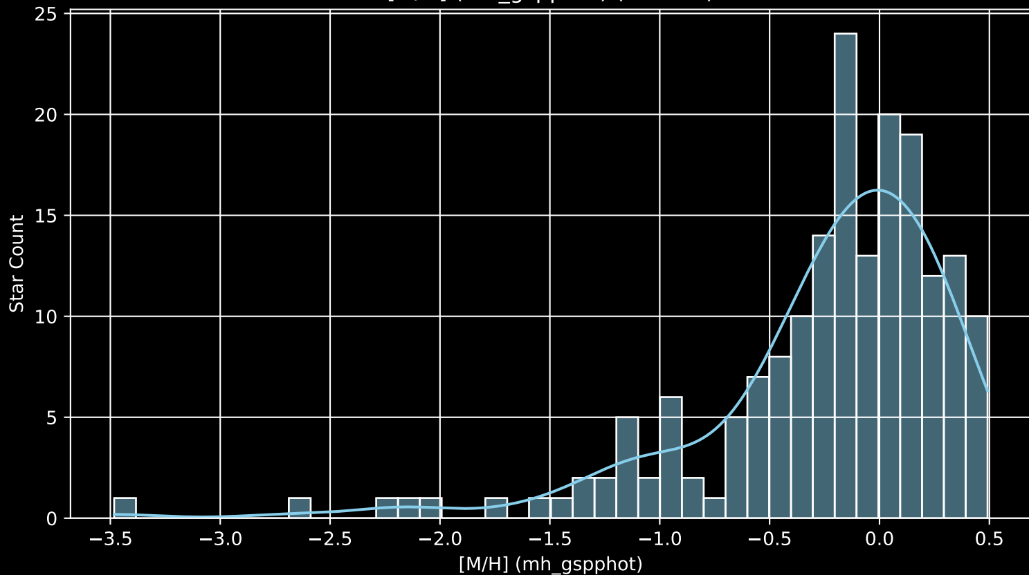
APOGEE DR17 Field: [355+04 [M/H] (mh_gspphot) (n= 183)
